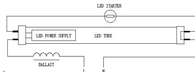
How to install * with magnetic ballast fixture installation
